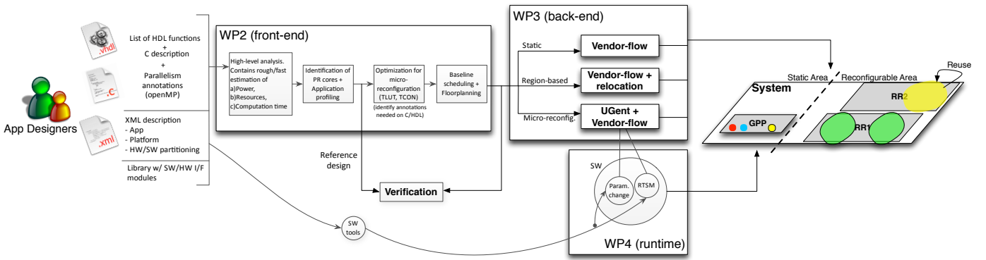
Fig. 1. FASTER design flow broken down into different parts
